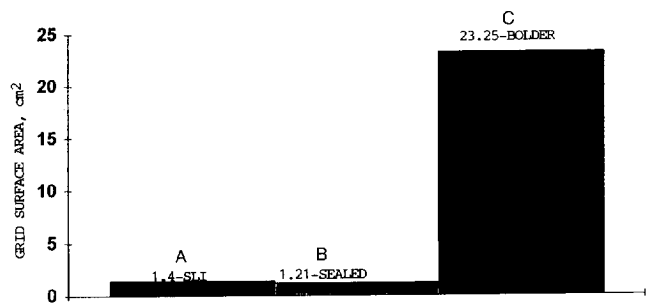
Fig. 1. Comparison of surface areas of grids (cm 2 ) per gram of active material: (A) SLI starter battery plate; (B) small valve-regulated (sealed) battery plate; (C) Bolder 1.2 Ah cell plate.
